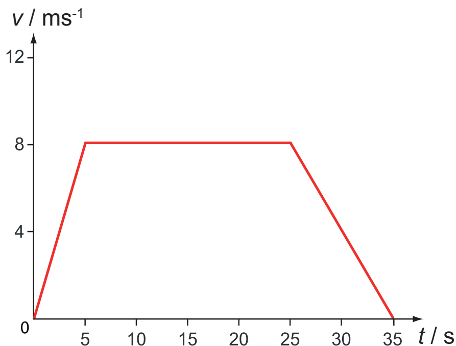
Figure 1.13: Velocity-time graph
