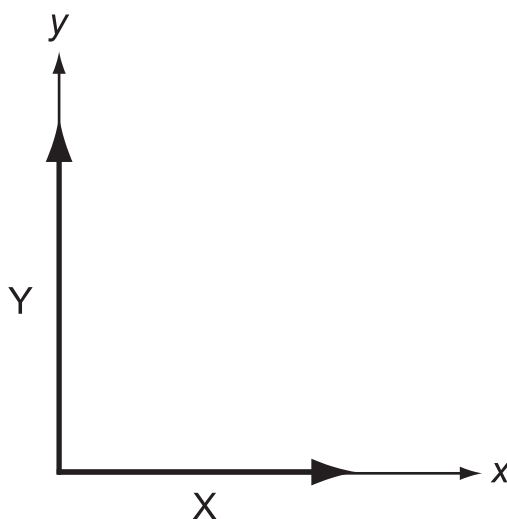
Figure 1.5: Perpendicular vectors
