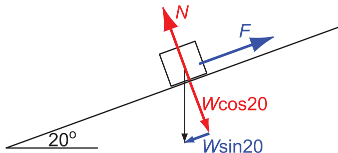
Figure 2.6: Free body diagram of the television on a tilted table
