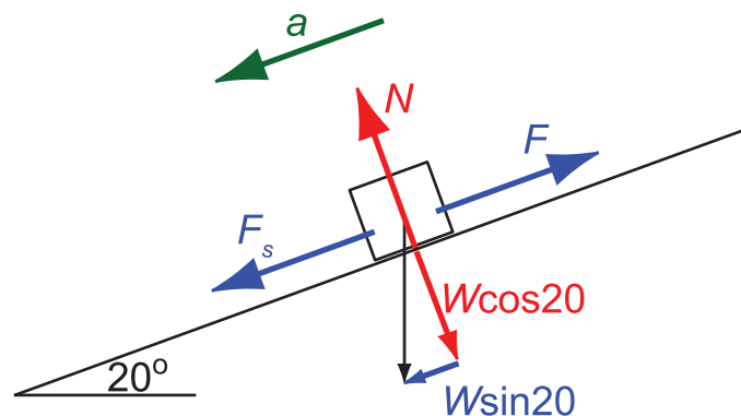
Figure 2.7: Free body diagram of the television sliding down the slope
