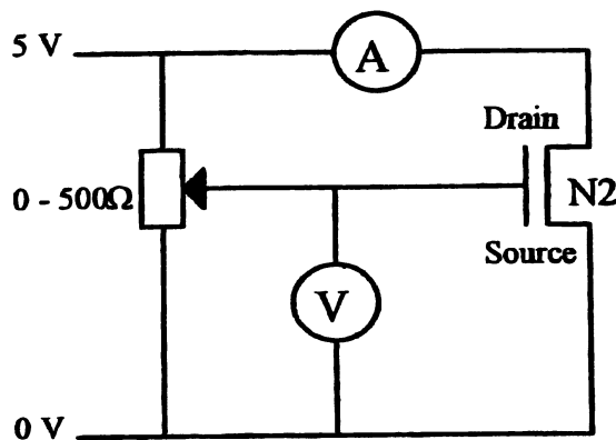
Circuit Diagram 1
